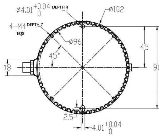
Figure 1.5 C32 Lidar Base
