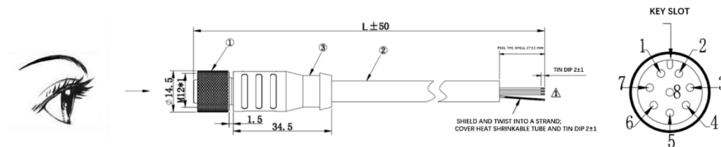
Figure 2.4 C32 Lidar Extension Cable (unit: mm)
