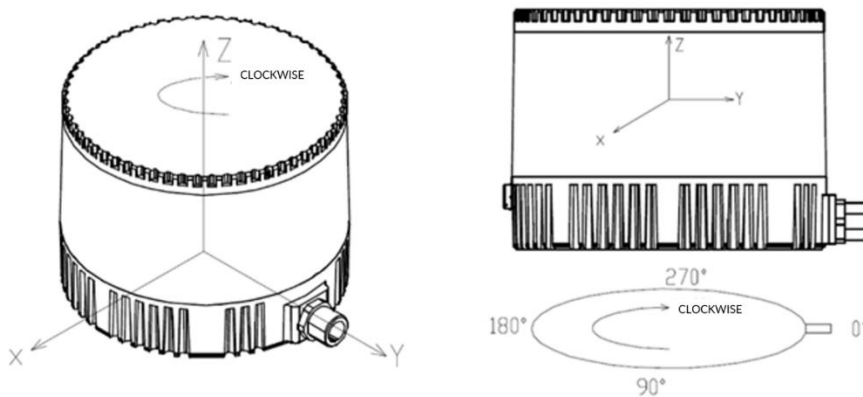
Figure 1.3 Coordinates & Scanning Direction
