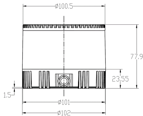
Figure 1.4 C32 Dimensions
