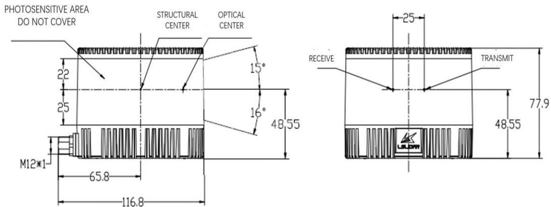
Figure 1.6 C32 Mechanical Drawing (unit: mm)
